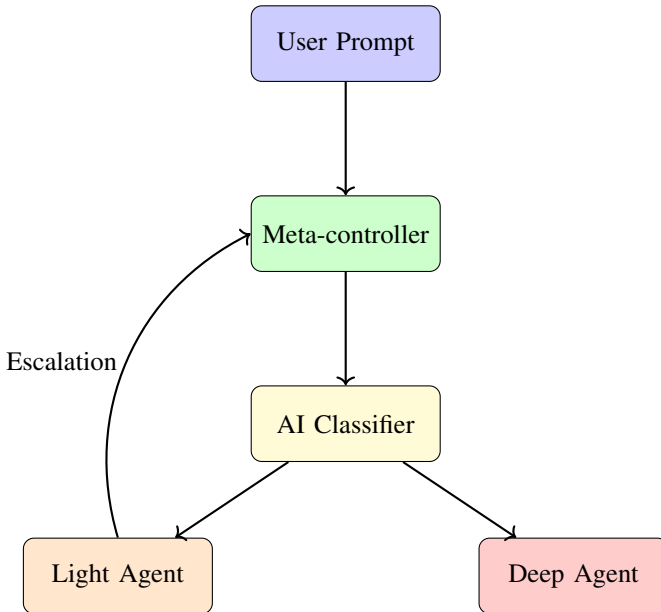
Fig. 1. Compact architecture of the Smart Meta-controller.
