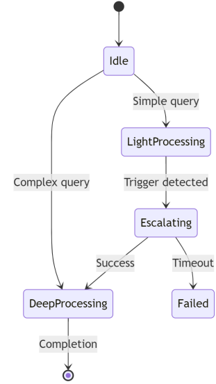
Fig. 2. Finite State Diagram of the Agent Orchestration
